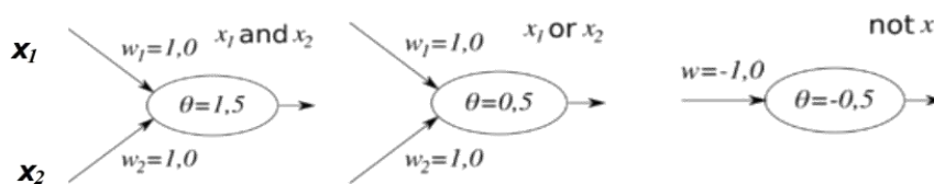
Figure 7 – Boolean functions
