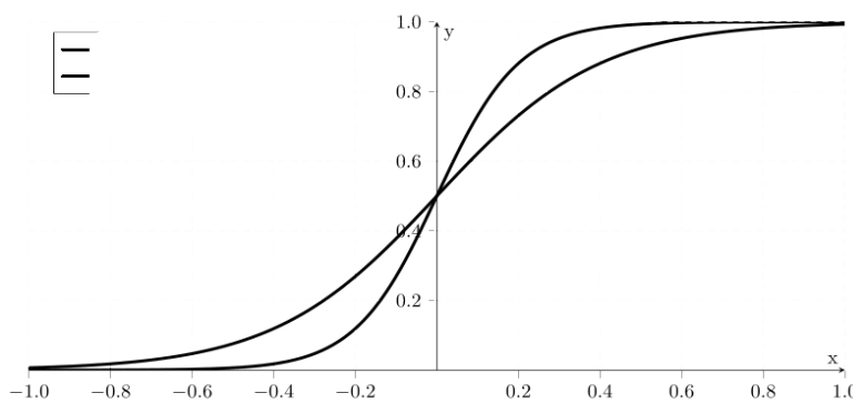
Figure 6 – Sigmoid function
