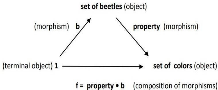
Figure 1 – Logical predicates
