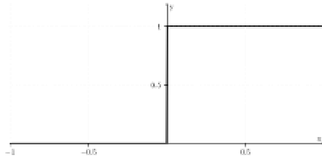
Figure 5 – Limit function
